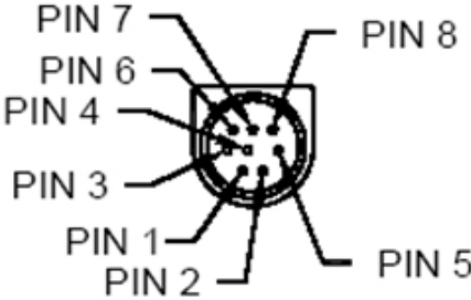
MINI-DIN 8 CONNECTOR
