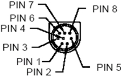
MINI-DIN 8 CONNECTOR
