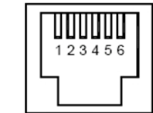
RS-232 Port from VFG
